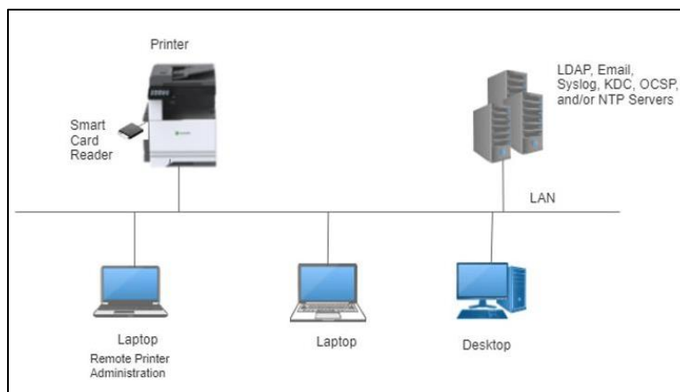
Figure 1: TOE Architecture
